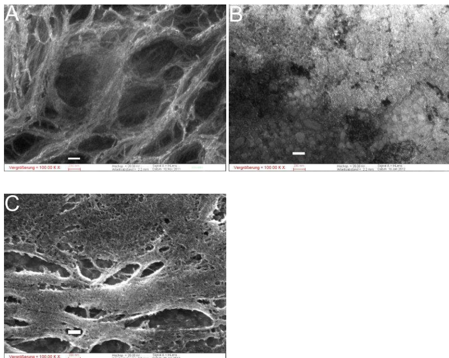
Figure S2. SEM images of (A) bundles of gold NWs produced by oleylamine synthesis and dispersed on a gold surface. The NWs were deposited from the hexane solutions, left to adhere overnight and washed three times with hexane. (B) As (A) but the solution of the NWs in hexane was subjected to US for 10 min before being deposited on the flat gold surface. (C) NWs after exposure to OP for 20 min (C). Scale bars are 200 nm.
